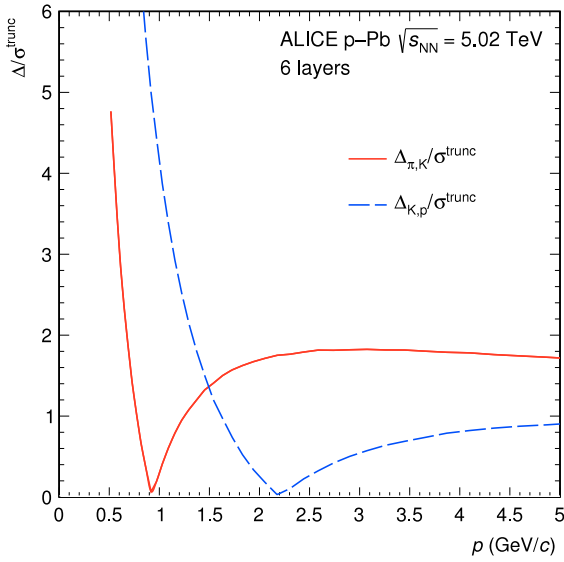
Fig. 40. Measured separation power ( \frac{\Delta}{\sigma^{trunc}} = \frac{S_{\pi,K}^{trunc} - S_{K,p}^{trunc}}{\sigma^{trunc}} ) for \pi/K and K/p separation as a function of momentum.
