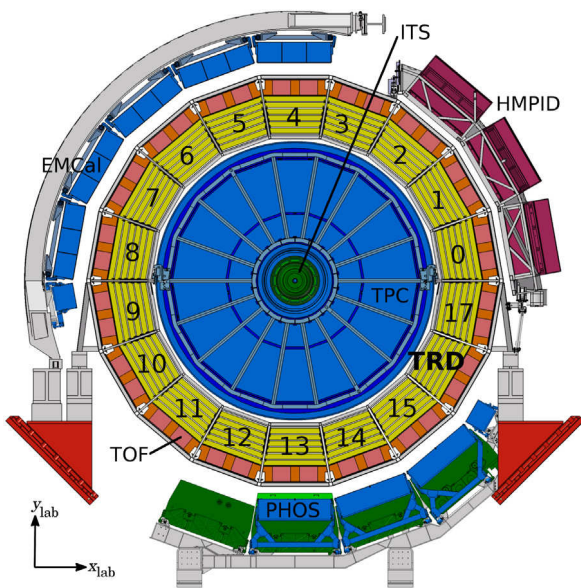
Fig. 1. Schematic cross-section of the ALICE detector perpendicular to the LHC beam direction (the start of LHC Run 2). The central barrel detectors cover the pseudorapidity range |\eta| \lesssim 0.9 and are located inside the solenoid magnet, which provides a magnetic field with strength B = 0.5 T along the beam direction.
